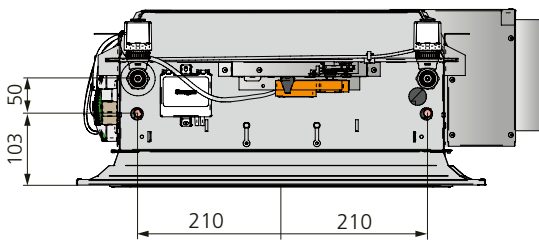
Figure 27. Dimensions, water connection length 600, 1200, 1800
