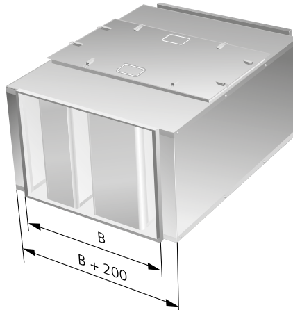
CALMO with cleaning hatch
