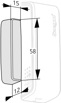
Figure 3. Dimensions, WISE WCS magnet.
