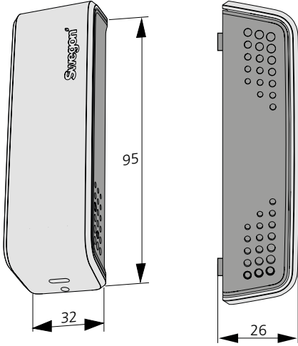
Figure 2. Dimensions, WISE WCS
