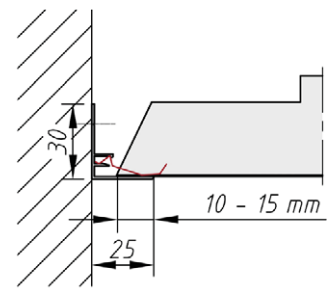
Support with trimming section for cut tile
