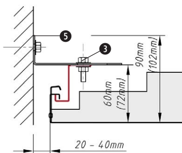
Wall mounting type A: with continuous wall bracket
