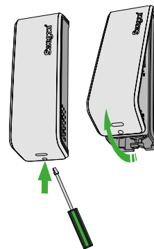
Figure 3a. Remove the front-piece. Always dismantle the product in this direction.
