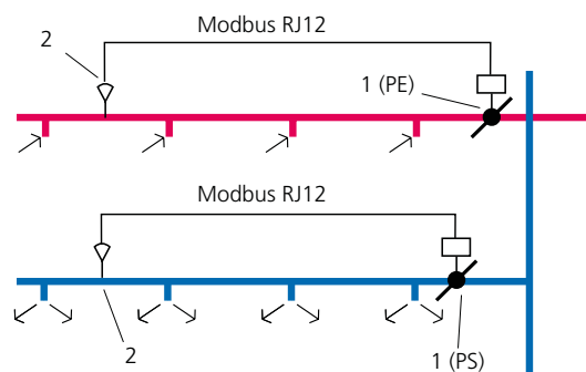
Figure 2. Constant pressure regulation, recommended installation 2/3 out in duct, max 100m.
