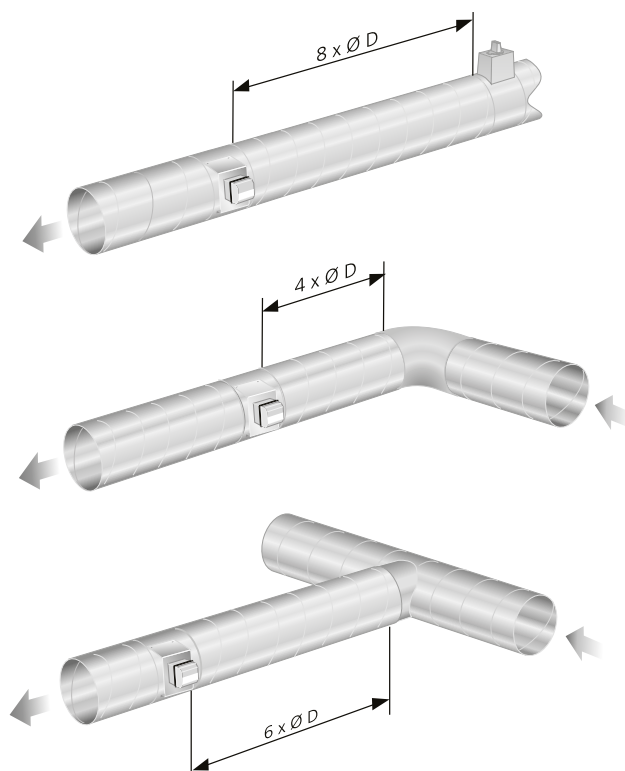
Figure 4. Straight section requirement before WISE DPS Modbus.
