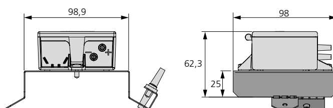
Figure 3. Dimensions, WISE DPS Modbus.
