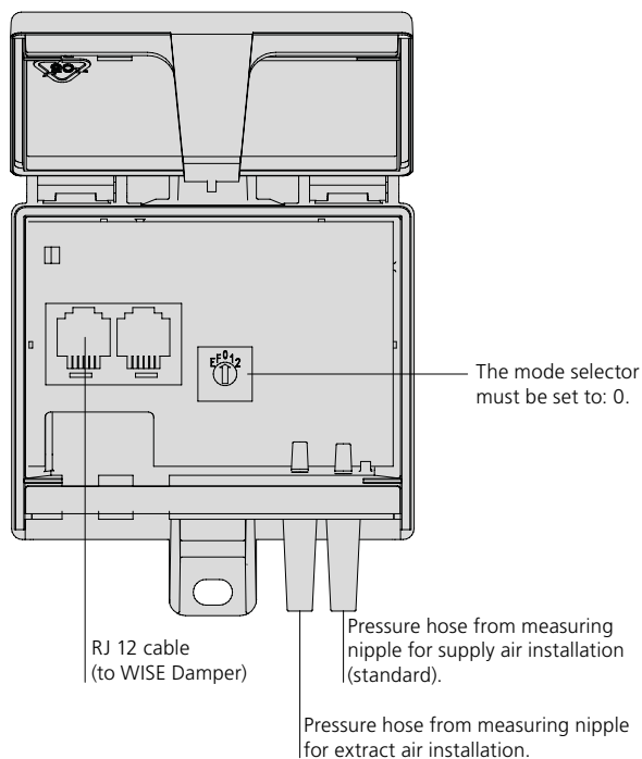
Figure 5. WISE DPS Modbus, connections.
