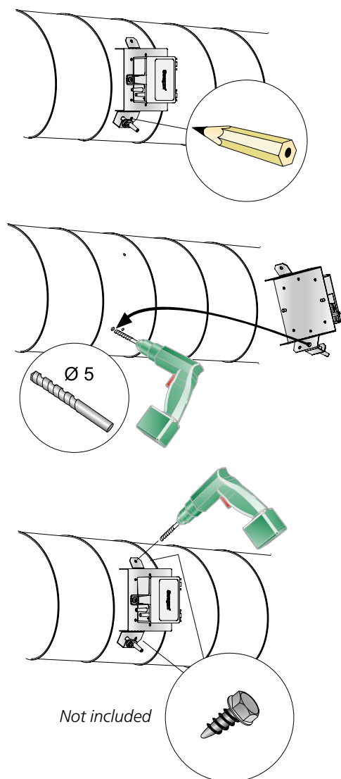
Figure 1. The pressure sensor shelf can be modified to fit the duct on which it is to be mounted, be it circular or rectangular.
